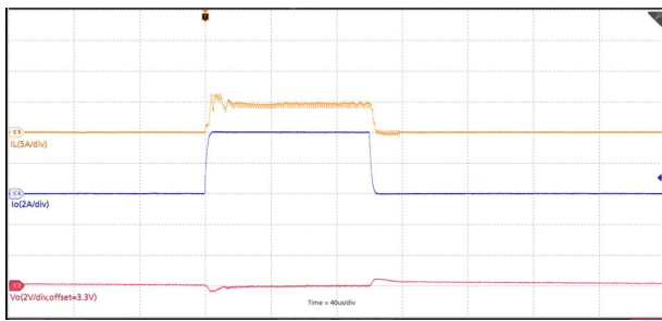
Figure 23. Overcurrent Protection
