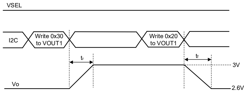
Figure 32 DVS Timing Using the I2C Interface
