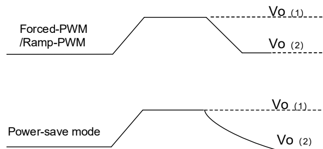
Figure 34 Ramp-PWM Operation
