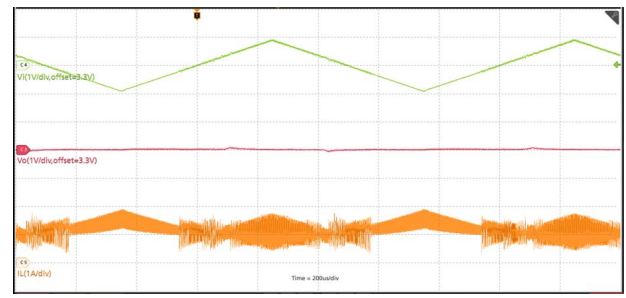
VIN=3.3V ± 0.9V, FPWM, T_A=25^{\circ}\text{C} , V_O=3.3\text{V} , R_L=3.3\Omega
