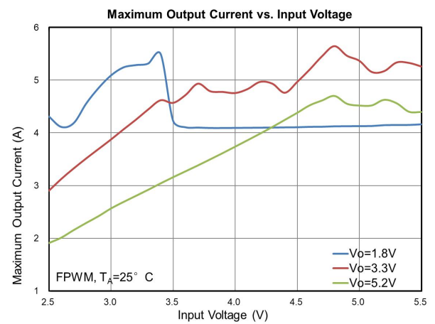
Figure 26. Maximum Output Current versus Input Voltage
