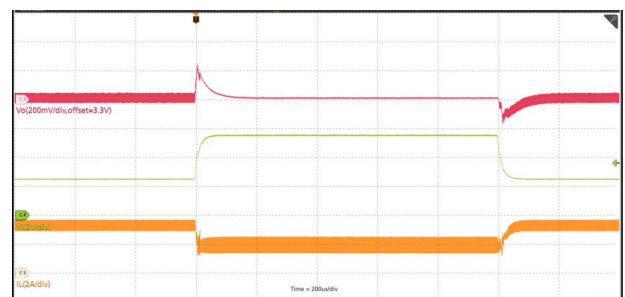
VIN=2.5V to 5.5V, PFM, T_A=25^\circ\text{C} , V_O=3.3\text{V} , I_O=2\text{A}
