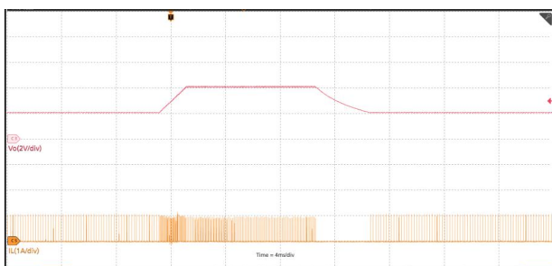
VIN=3.6V, PFM, T_A=25^{\circ}\text{C} , V_O=2\text{V} to 4V, R_L=330\Omega
