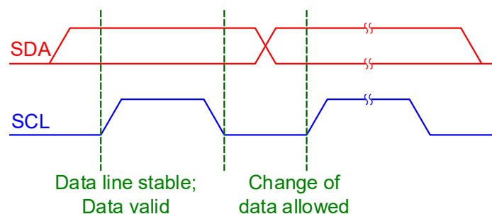
Figure 36 Bit Transfer on the Serial Interface
