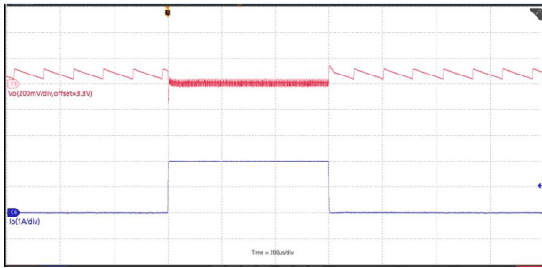
VIN=4.2V, PFM, T_A=25^{\circ}\text{C} , V_O=3.3\text{V} , I_O=10\text{mA} to 2A
