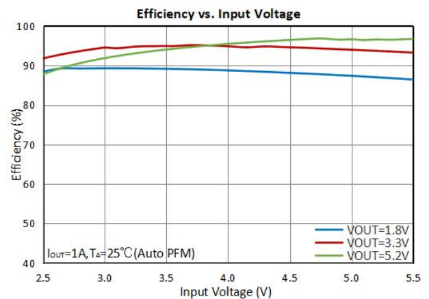
Figure 4 Efficiency versus Input Voltage (ultra-sonic enable)
