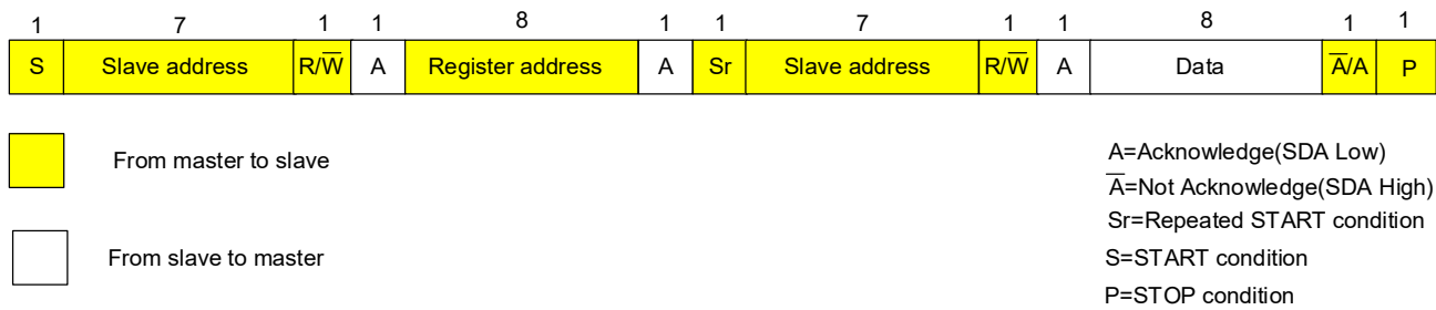
Figure 40 Read Data Transfer Format in Standard, Fast and Fast-Plus Modes
