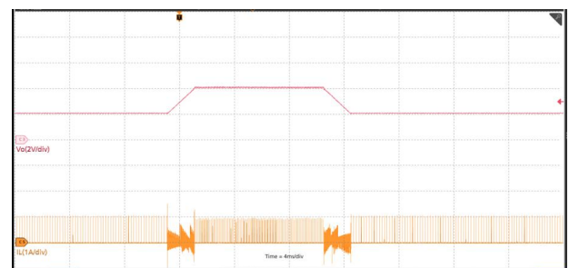
VIN=3.6V, PFM, T_A=25^{\circ}\text{C} , V_O=2\text{V} to 4V, RPWM, R_L=330\Omega
