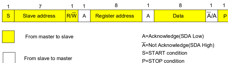
Figure 39 Write Data Transfer Format in Standard, Fast and Fast-Plus Modes
