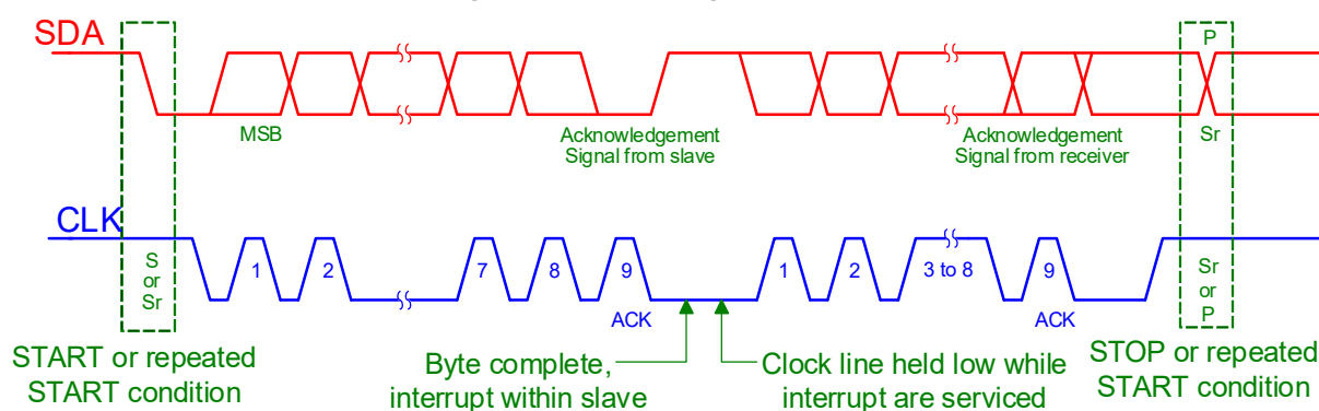
Figure 38 Bus Protocol
