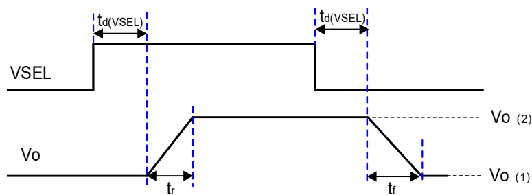
Figure 31 DVS Timing Diagram Using the VSEL Pin
