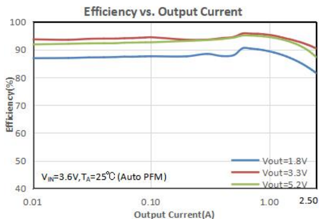
Figure 3 Efficiency versus Output Current (ultra-sonic enable)
