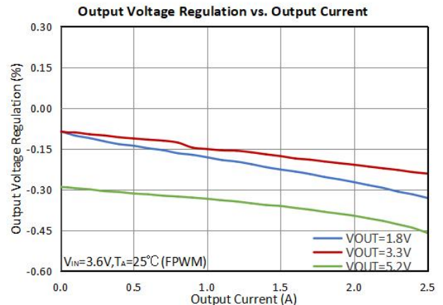
Figure 6. Load Regulation
