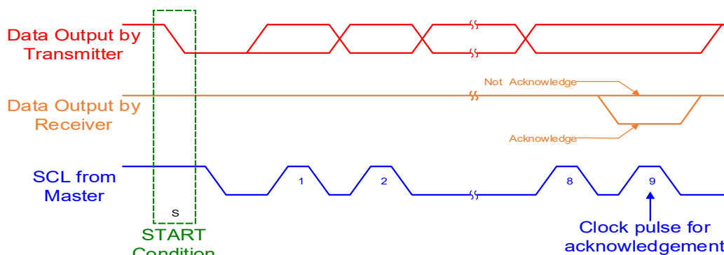
Figure 37 Acknowledge on I2C Bus
