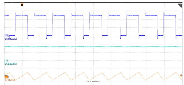
VIN=5V, FPWM, T_A=25^\circ\text{C} , V_O=3.3\text{V} , I_O=100\text{mA}
