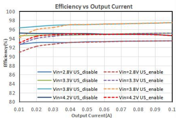
Figure 27. Efficiency versus Output Current (Ultra-sonic enable VS disable)
