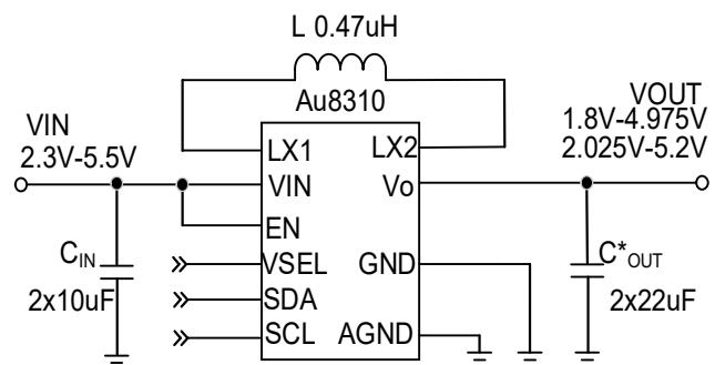
Figure 1 Simplified Schematic
