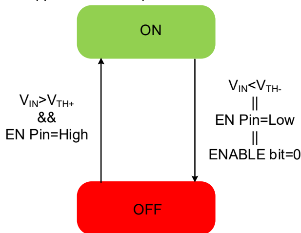
Figure 33 Device Functional Modes
