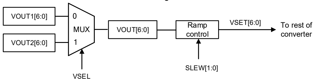
Figure 30 Dynamic Voltage Scaling Block Diagram
