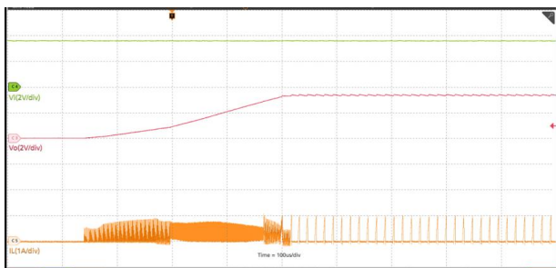
VIN=3.6V, PFM, T_A=25^{\circ}\text{C} , V_O=3.3\text{V} , R_L=33\Omega
