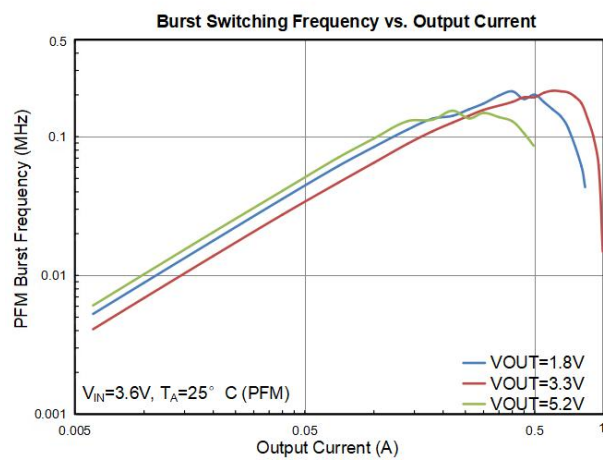
Figure 25. Burst Switching Frequency versus Output Current
