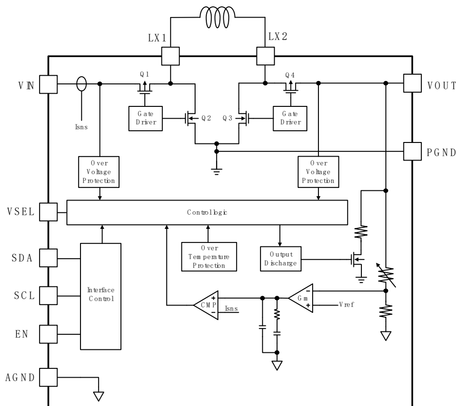
Figure 28 Block diagram
