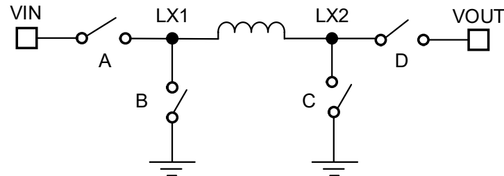
Figure 29 Buck-Boost Topology
