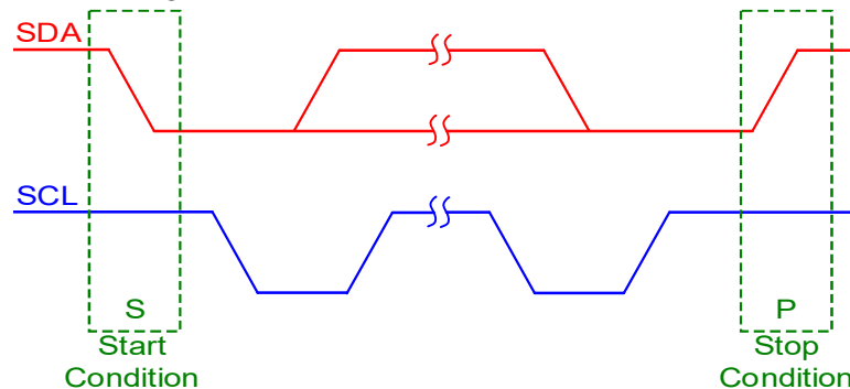
Figure 35 START and STOP Conditions
