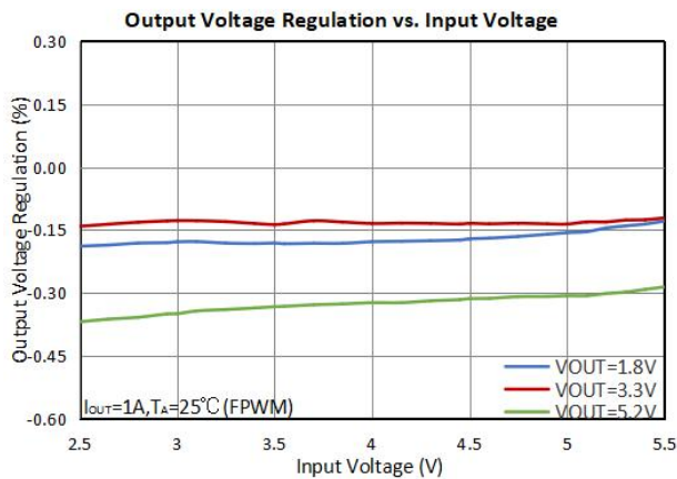
Figure 5. Line Regulation
