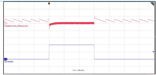
VIN=3.3V, PFM, T_A=25^{\circ}\text{C} , V_O=3.3\text{V} , I_O=10\text{mA} to 2A
