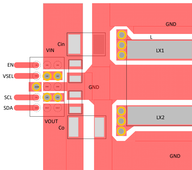
Figure 42 Layout Example
